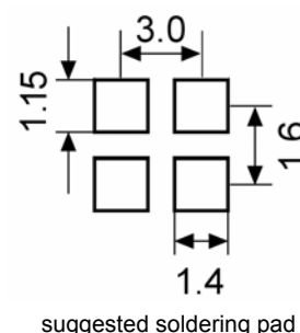
suggested soldering pad
